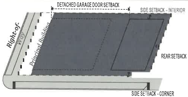
ACCESSORY BUILDING SETBACKS (2.4.1.C)
